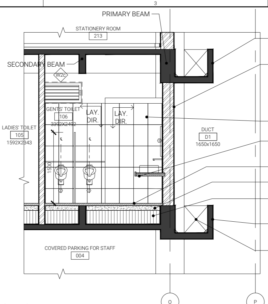
2 SECTION 8 1:50
