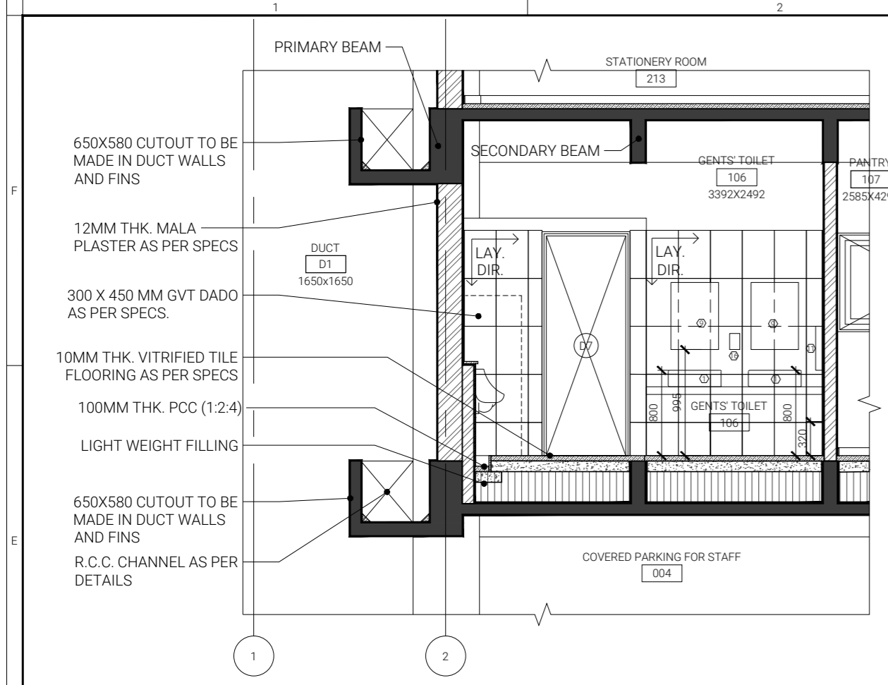
1 SECTION 7 1:50
